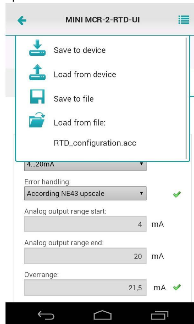
Figure 20 Communication menu
